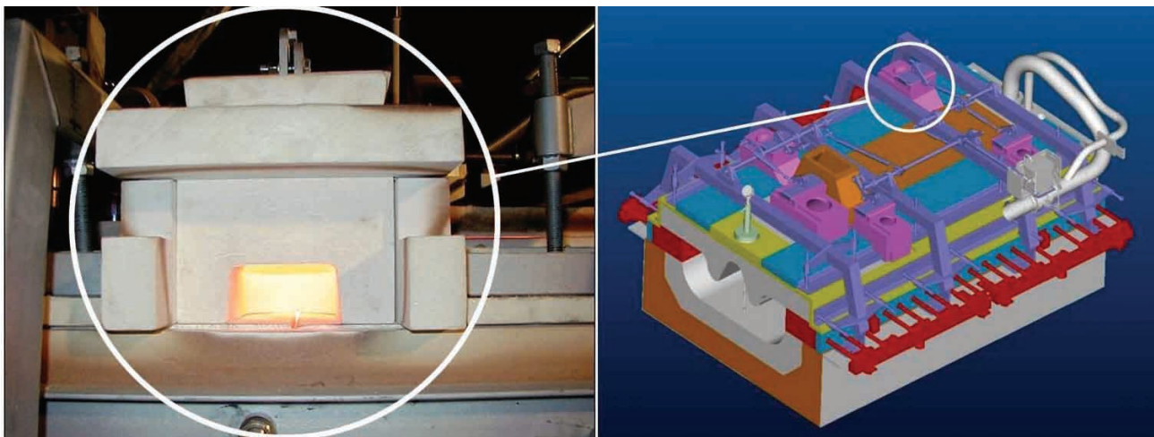
Fig. 2 - The 340 Forehearth flue exhaust control.
