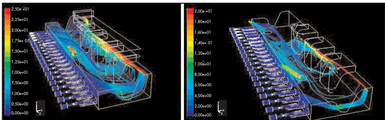
Fig. 1 - Models of three-flue & five-flue forehearth configurations.
