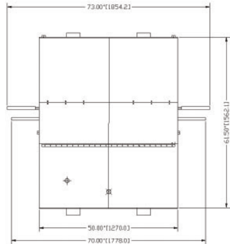
Shown without Bottle Spacer or Ware Transporter
