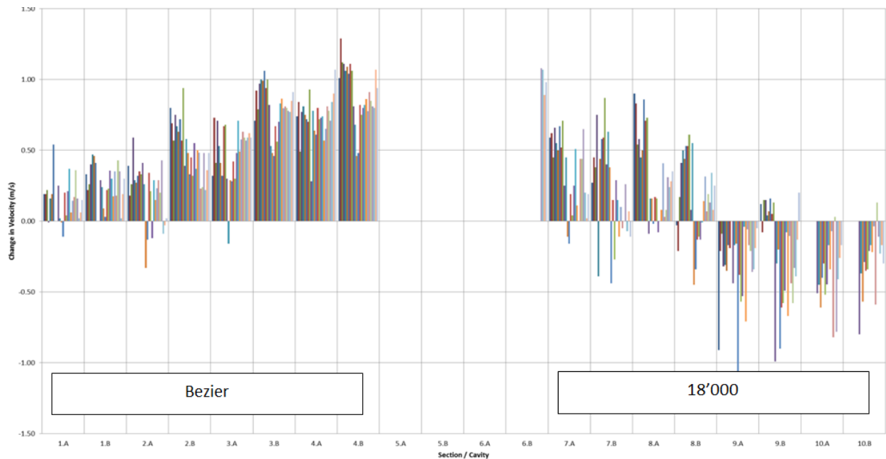
Picture 4: Changes in velocity Bezier Vs previous delivery from field trials on a 10 sections machine. Negative values means that gobs are decelerating during their transition through the delivery equipment.
