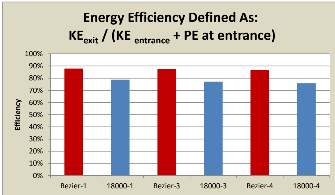
Picture 3: comparison of Energy efficiency between Bezier and conventional deflectors. The Bezier curve and the longer landing zone creates less Kinetic energy dissipation during the transition in the deflectors.
